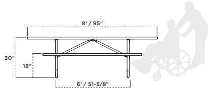
158H-PT8 8' Double-Sided ADA Accessible Table, portable, pressure treated planks, galvanized frame
