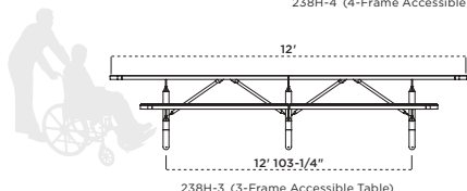
238H-3 (3-Frame Accessible Table)
