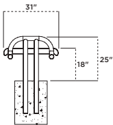
02B-976SM-V4 4' Contour Cantilevered Bench without Back, surface mount, blue diamond pattern, black frame
