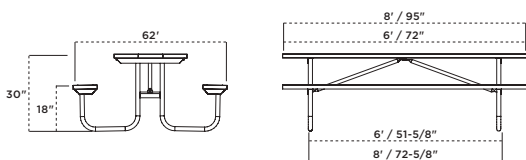
158-GRY6 6' Heavy-Duty Rectangular Table, portable, grey recycled plastic planks, black frame
