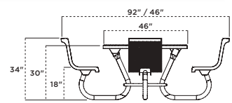
230-RDPC-46 46" Round Contour Table, brown perforated pattern, brown frame
