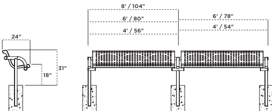
02B-975SM-W6 6' Contour Cantilevered Bench with Back, surface mount, red wave pattern, white frame
