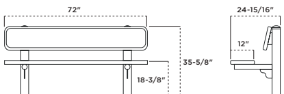
02B-961SM-V6 6' Single-Sided Bollard Bench, surface mount, red diamond pattern, black frame
