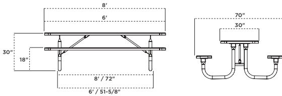
238-V8 8' Extra Heavy-Duty Rectangular Table, brown diamond pattern, white frame
