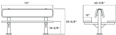
02B-962SM-V6 6' Double-Sided Bollard Bench, surface mount, ultra blue diamond pattern, ultra blue frame
