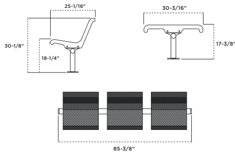
02B -800P-VS3 -3-Seat Straight Bench with Back, portable, brown diamond pattern, brown frame
