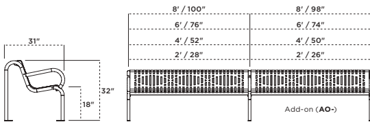
O2B-955SM-W6 6' Sierra Bench, surface mount, red wave pattern, red frame
