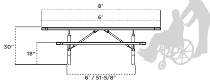
238H-V8 8' Double-Sided ADA Accessible Table, red diamond pattern, black frame
