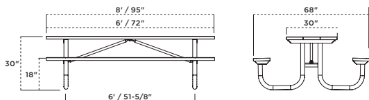
238-GRN6 6' Extra Heavy-Duty Rectangular Table, green recycled plastic planks, portable, galvanized frame
