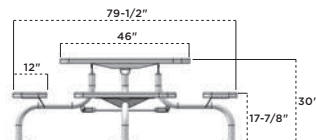
369SM-V Square Lion Outdoor® Span Leg Table, black diamond pattern, black frame
