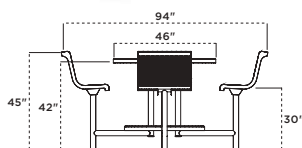
362SM-RDV 46" Lion Bar Height Table, surface mount, ultra blue diamond pattern, ultra blue frame
