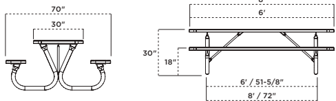
BT238-V6 6' Extra Heavy-Duty Bolt-thru Rectangular Table, green diamond pattern, black frame
